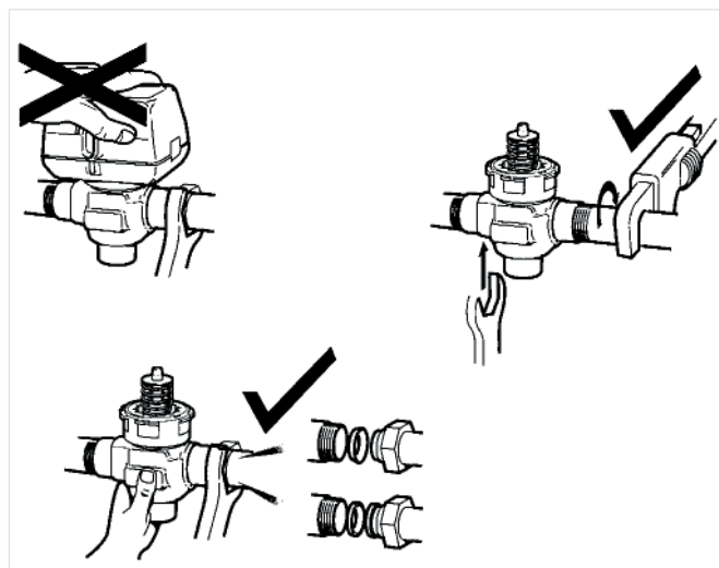
Fig. 5 Plumbing
