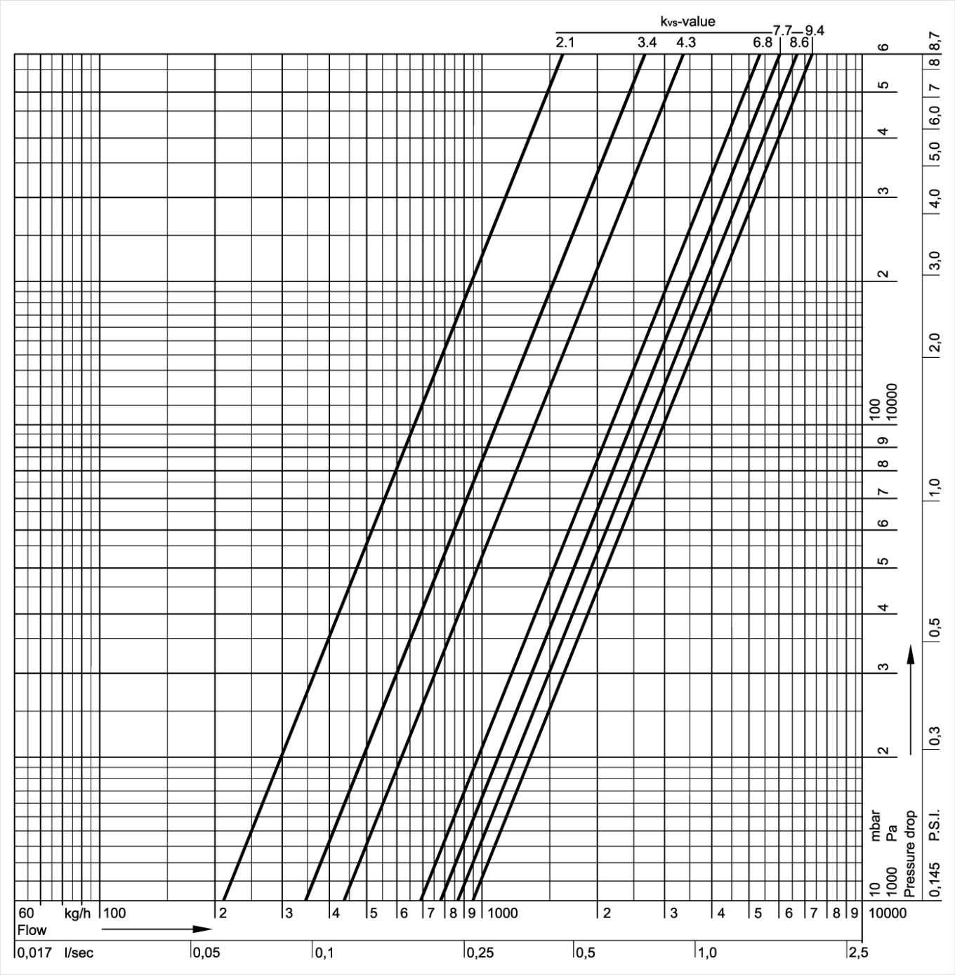
Fig. 7 Valve pressure loss characteristic
